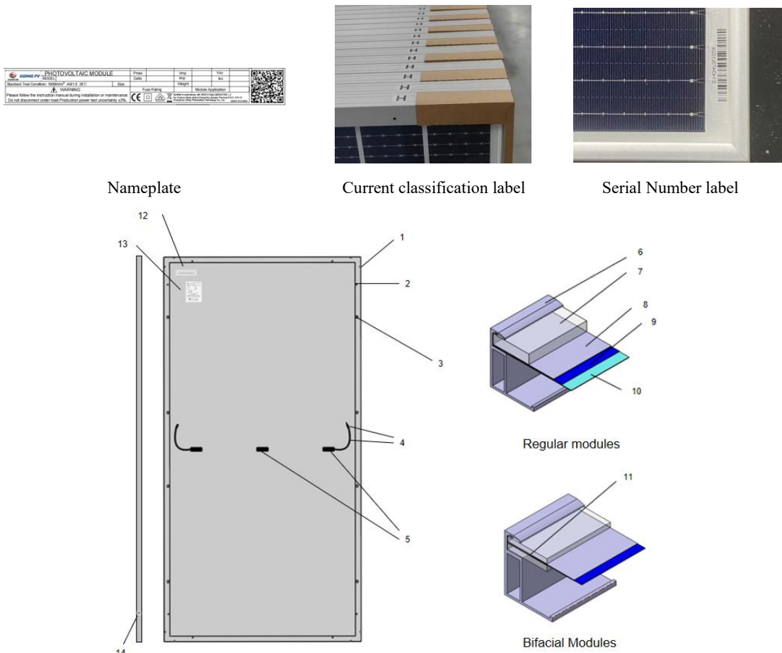
Figure 1 Regular Modules Mechanical Drawing
