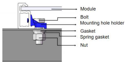
Sectional view
